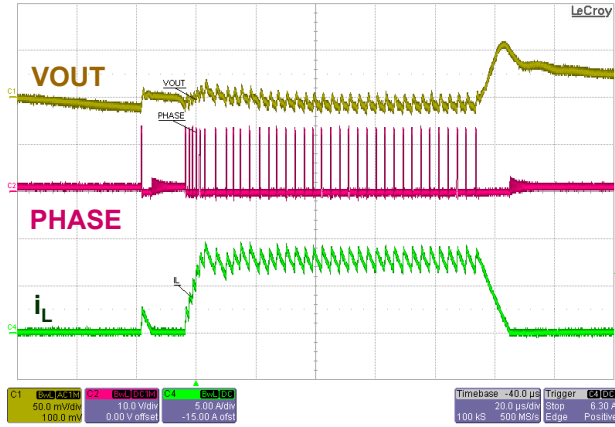
50mV/div 10V/div 5A/div 20µs/div Fig. 15: Load Transient 0-8A
