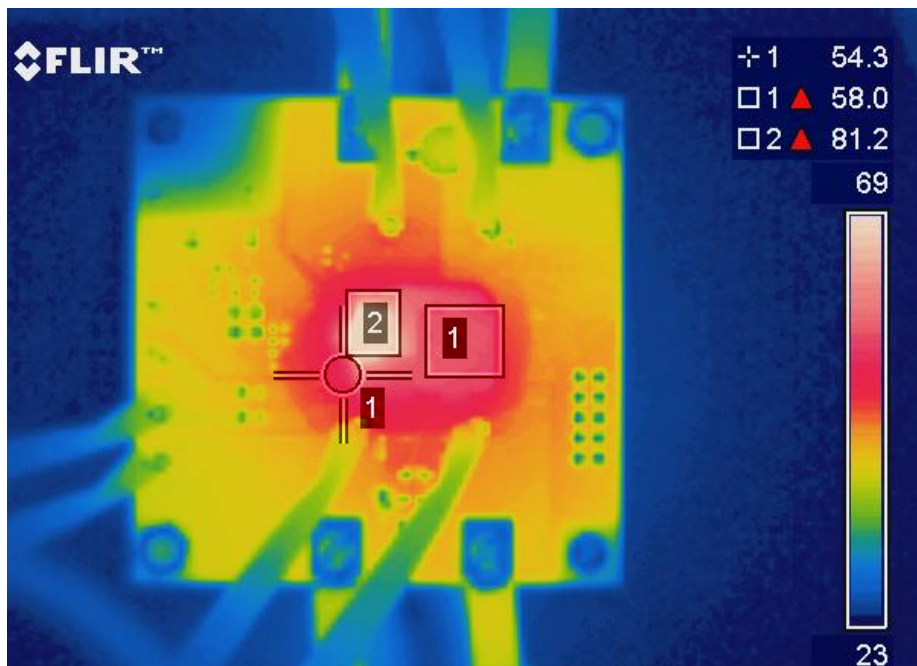
Fig. 17: Thermal Image (IR3876: 81°C, Inductor: 58°C, PCB: 54°C)
