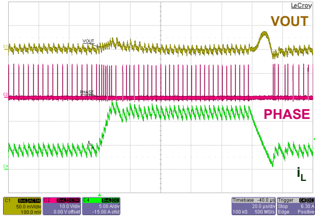
50mV/div 10V/div 5A/div 20µs/div Fig. 16: Load Transient 4-12A
